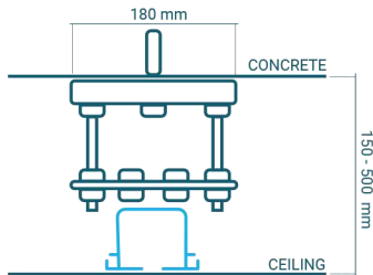
BENT PLATE
