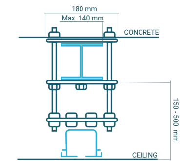
STEEL BEAM WITH 3 PLATES
